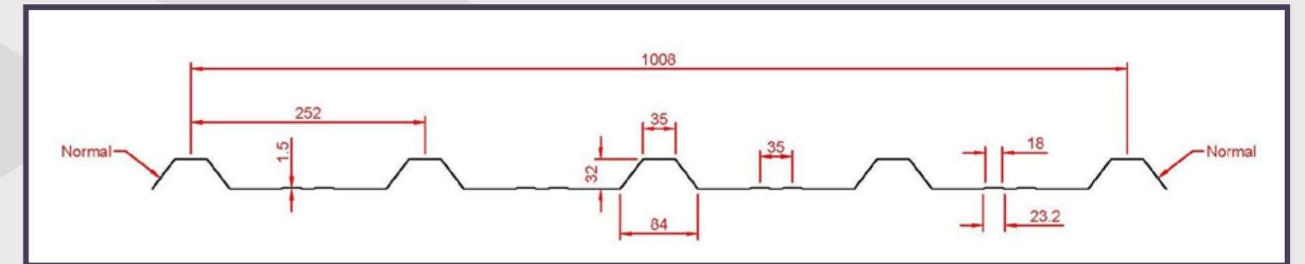
CS 32/1000 Box Profile. Available from 1.2m/4ft up to 7.35m/24ft (1000mm cover)
