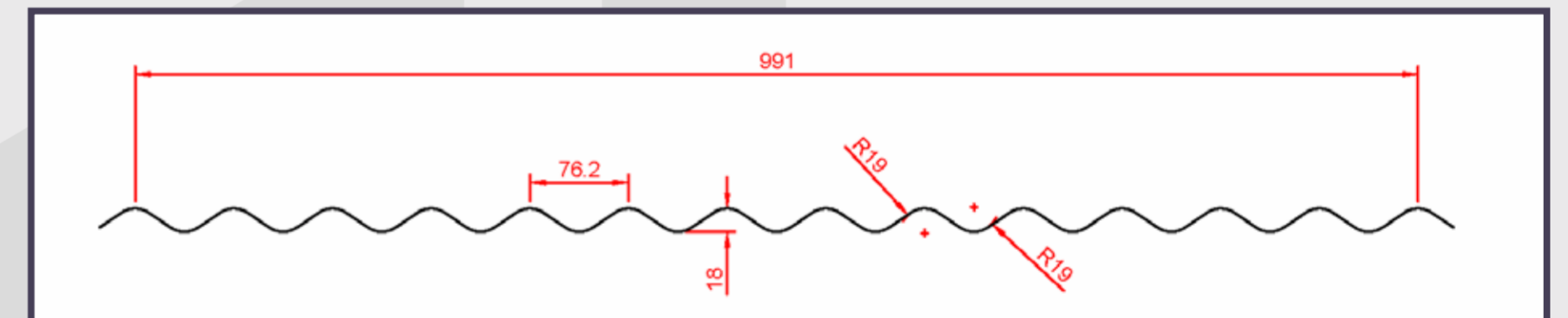
CS 13/3 Corrugated. Available from 1.2m/4ft up to 7.35m/24ft (990mm cover)
