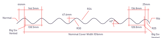
Big 6 Rooflight
