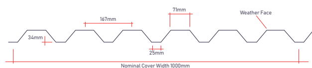
34/1000 Box Profile Wall
